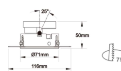
Adaptador de techo RA22 Ref. BL-ACC-RA22-DWX1
